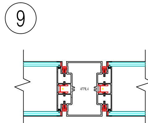
9 3" In-Line Post
