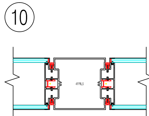
10 4" In-Line Post
