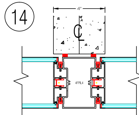
14 3" In-Line Post at 4" Drywall Bypass
