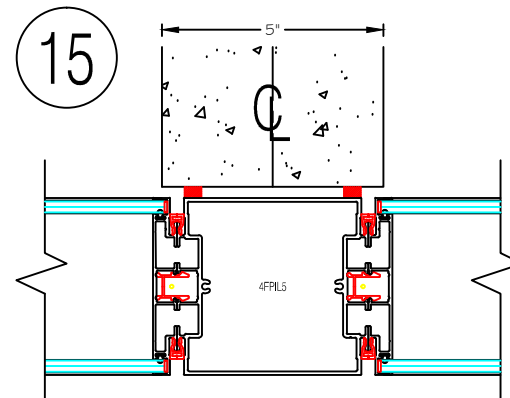
15 4" In-Line Post at 5" Drywall Bypass
