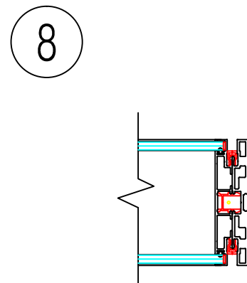
8 Finished End
