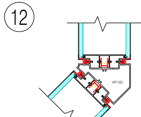
12 135 Degree Post
