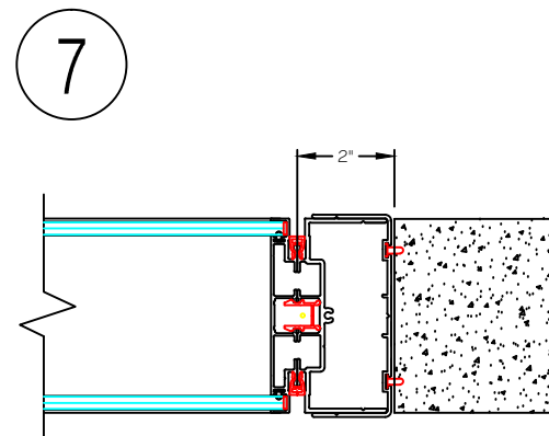
7 2" Mini-End
