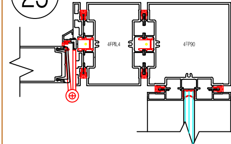
DF @ Post 90 Degree Swing Aluminum Door
