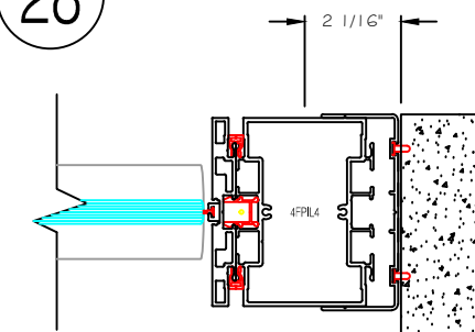
Center Pivot Glass Door @ 3.5" ME
