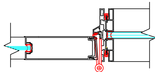
Panel to DF Hinge Aluminum Door
