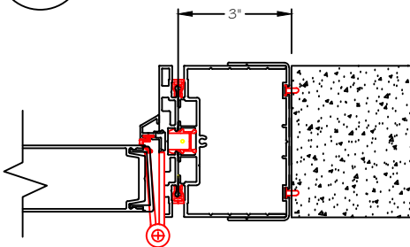
DF @ 3" Mini-End Aluminum Door
