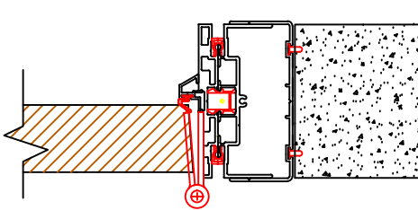
DF @ 2" Mini-End Wood Door
