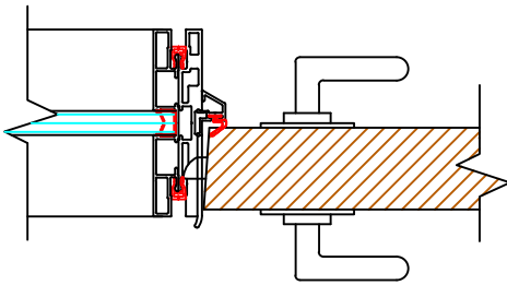
Panel to DF Keeper Wood Door
