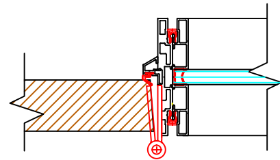
Panel to DF Hinge Wood Door
