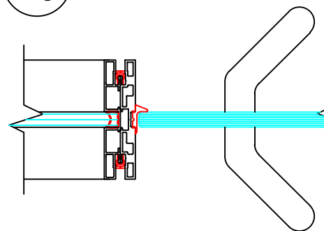
Panel to Center Pivot Glass Door @ Keeper
