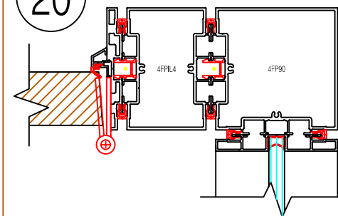
DF @ Post 90 Degree Swing Wood Door
