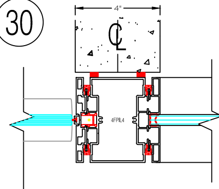
Center Pivot Glass Door @ In-Line Post
