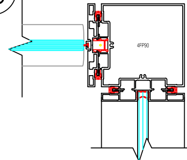
Center Pivot Glass Door @ 2-Way Post
