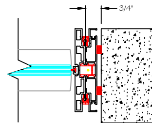
Center Pivot Glass Door @ Flush WS
