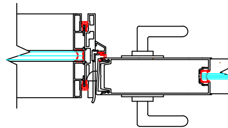
Panel to DF Keeper Aluminum Door
