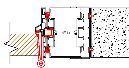
DF @ 3.5" Mini-End Wood Door
